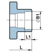
SOCKET WELD END
