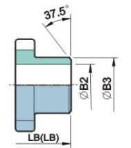
LB (Butt-welding End) LE (Extended Butt-welding End)
