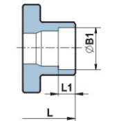
SOCKET WELD END
