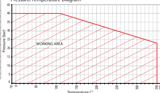
Pressure/Temperature Diagram
